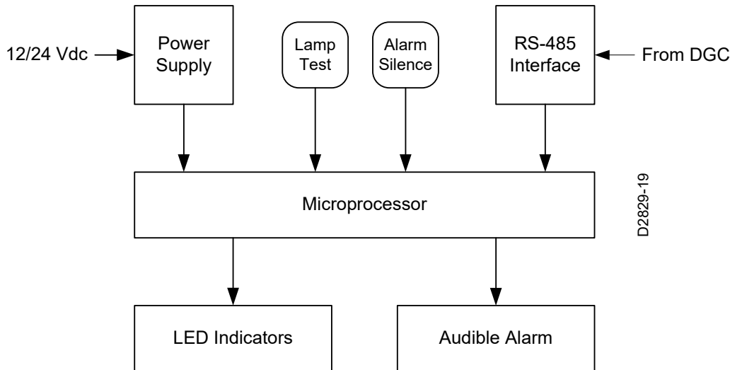
Figure 2. RDP-110C Function Blocks
