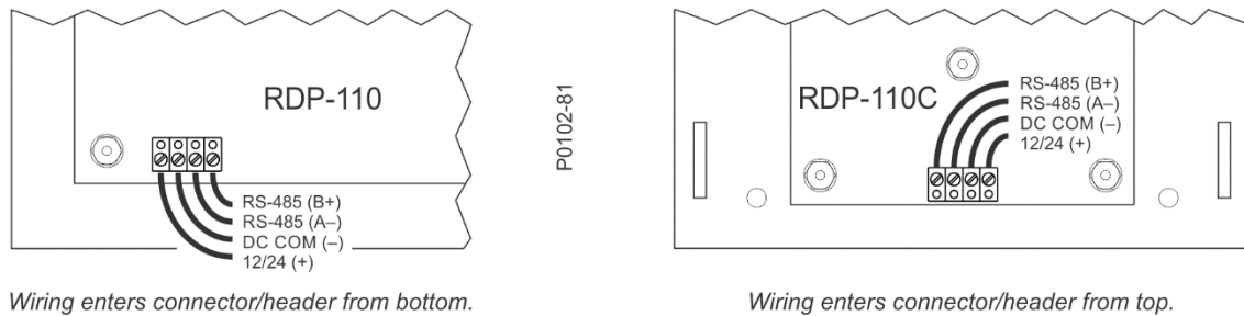
Figure 9. RDP-110/RDP-110C Wiring Differences
