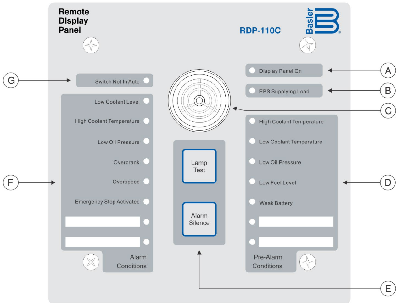
Figure 3. Controls and Indicators
