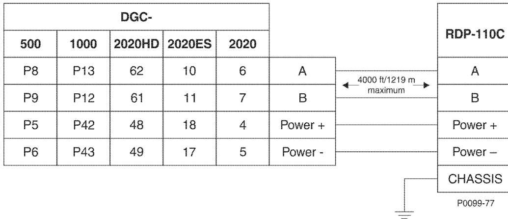
Figure 11. Typical Connections
