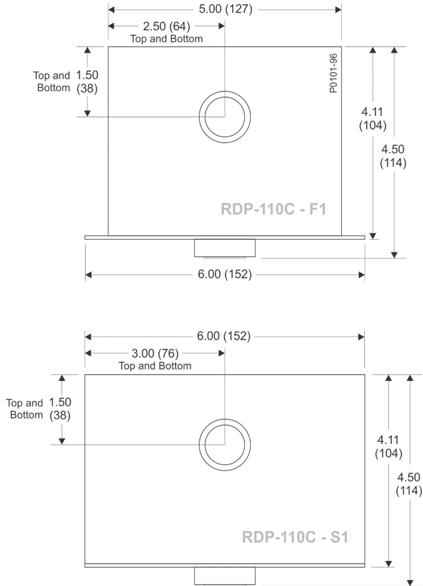
Figure 7. Mounting Dimensions and Knockout Locations, Top and Bottom, F1 and S1 Styles
