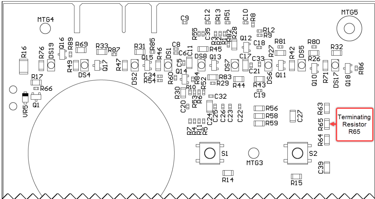
Figure 10. RS-485 Terminating Resistor Location
