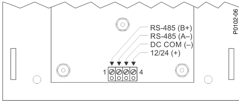
Figure 8. Circuit Board Connections
