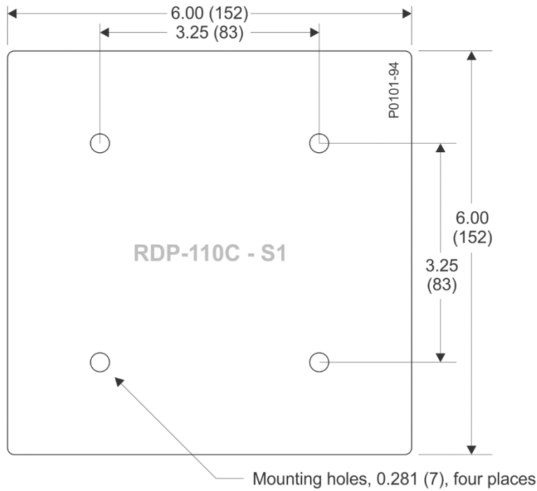
Figure 5. Mounting Dimensions, Rear, F1 and S1 Styles
