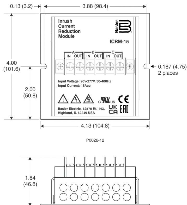
Figure 1. Dimensions ICRM
