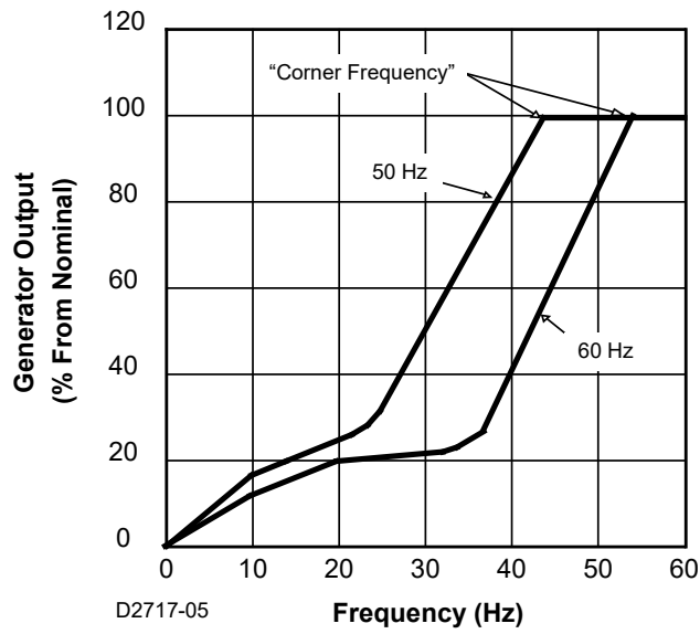
Figure 1. Frequency Compensation Curves
