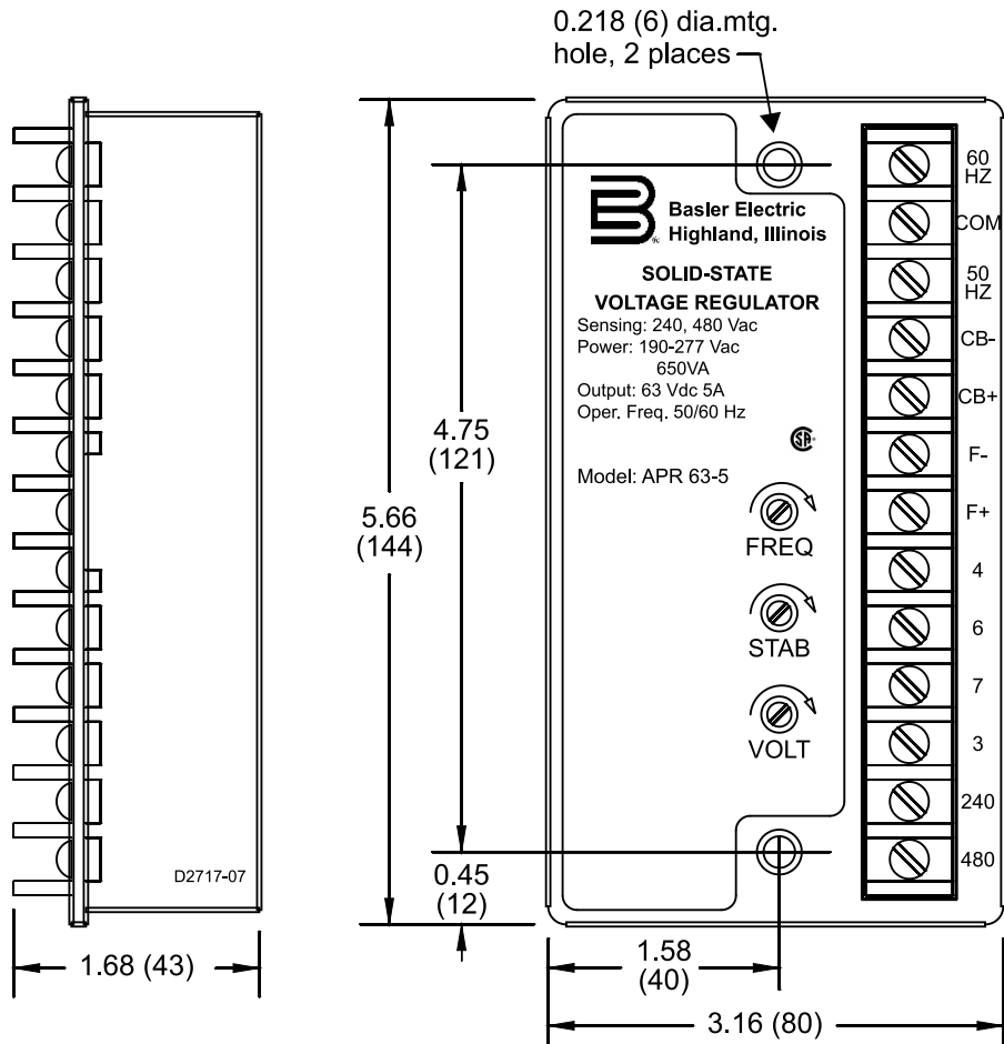
Figure 3. APR 63-5 Mounting Dimensions and Controls Illustration
