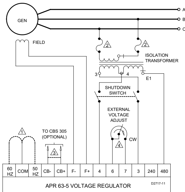
Figure 5. Typical Connections for 480 Vac
