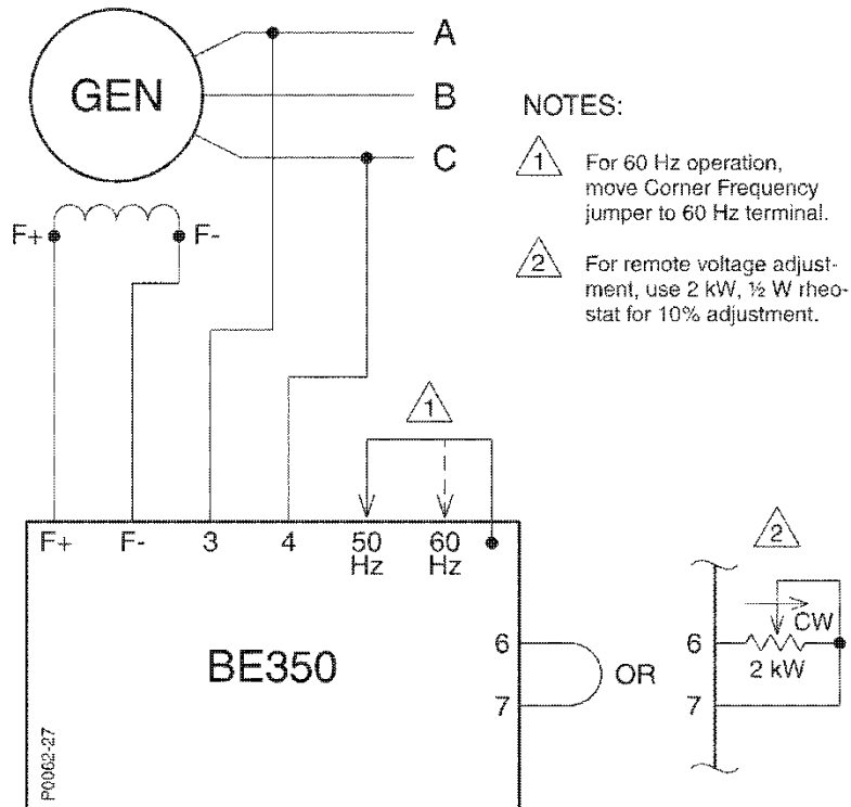
Figure 5. Typical Connections
