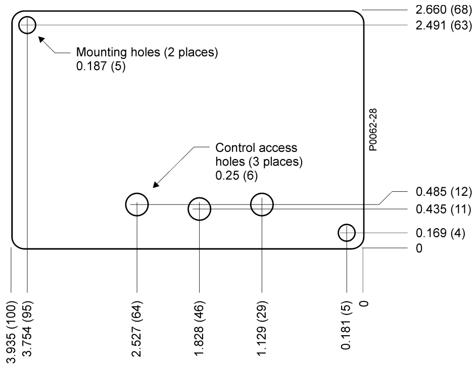
Figure 4. Panel Drilling and Mounting Dimensions
