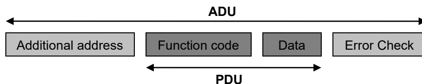
Figure 1-1. General Modbus Frame
