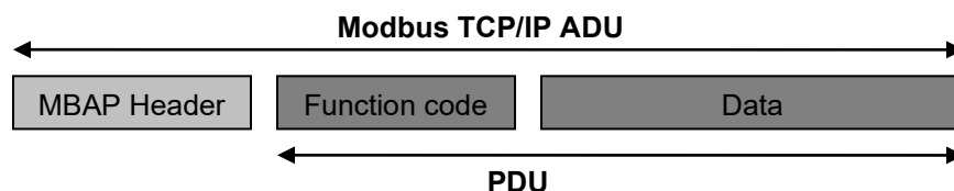
Figure 1-2. Modbus Request/Response Over TCP/IP
