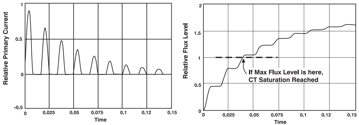
Figure 5: Point where CT saturation is reached
