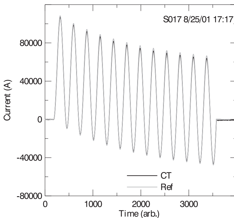
Figure 13: Fully Offset 40 \text{ kA}_{\text{RMS}} , 108 \text{ kA}_{\text{peak}} Fault Current – 12 Cycle Duration
