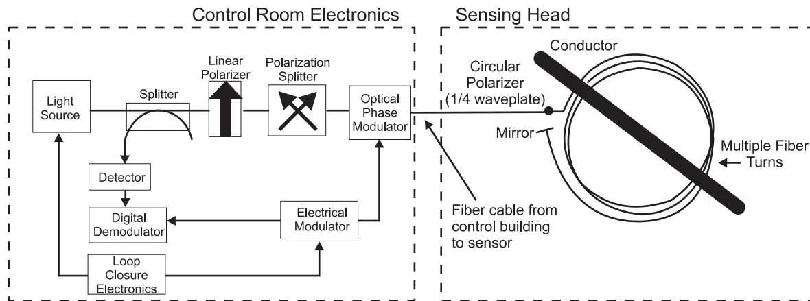
Figure 11: Fiber optic current sensing technology. Circularly polarized light travels in both directions around the fiber loop with speed of propagation differentially influenced by the Faraday effect. The signal is normalized and bifurcated with a modulator and closed loop electronics to yield a highly accurate current measurement impervious to temperature and vibration effects.
