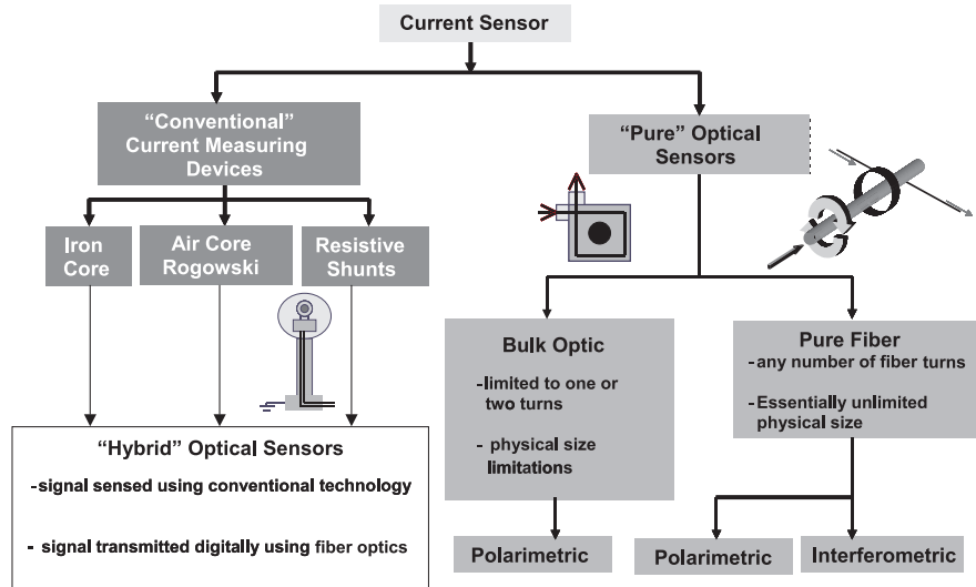
Figure 8: An overview of major categories of current sensing approaches on the market
