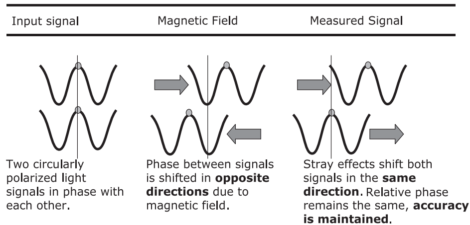
Figure 10: Interferometric CTs measure the difference between polarization shift of two signals caused by the current in a conductor.
