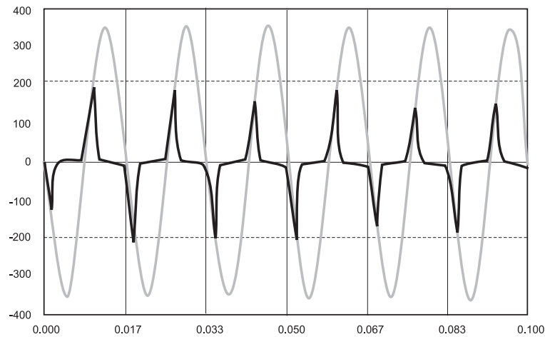
Figure 6: 600:5 tapped at 200:5; C200 effectively a C65; 1.2+j.2 \Omega burden total
