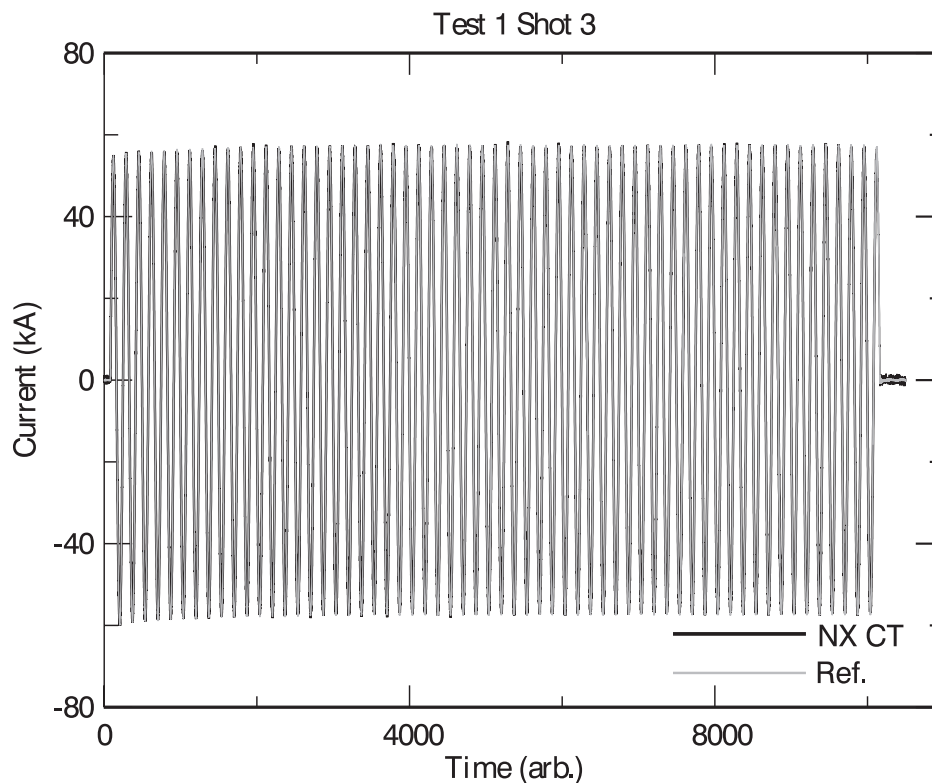
Figure 14: Symmetrical 40kA RMS Thermal Fault Current Test – One Second Duration
