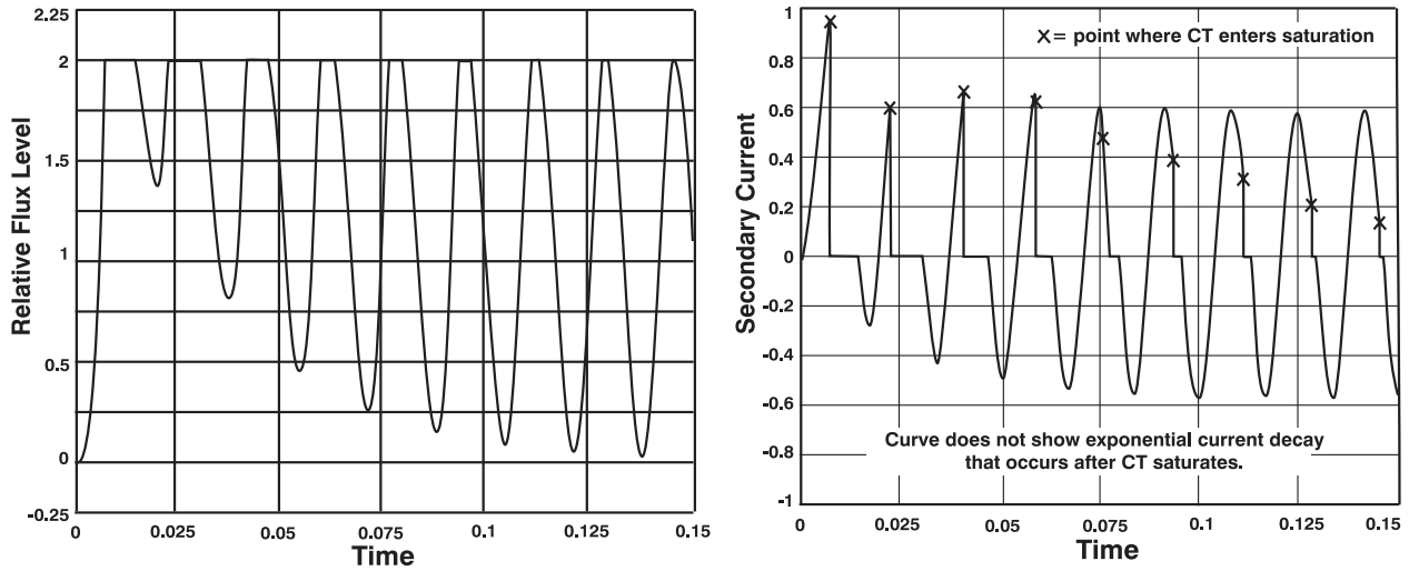
Figure 4: Simplified Saturation Effects Analysis
