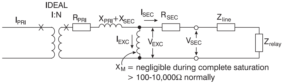
Figure 1: Simplified CT Equivalent Circuit
