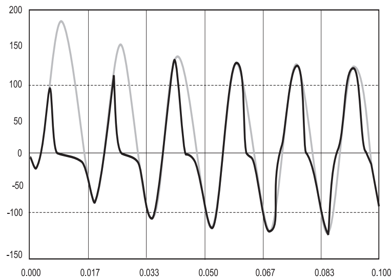
Figure 7: Same CT, tapped at 600:5, but with heavy DC offset
