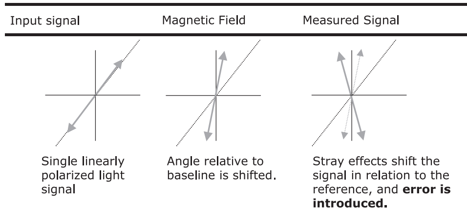
Figure 9: Polarimetric CTs measure the magnitude of a shift in the polarization of light caused by the current in a conductor.
