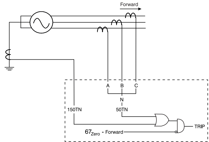
Fig. 17. Ground Fault Sensing Schematic
