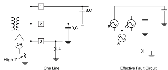
Fig. 18. Line to Ground Fault on High Z_G System
