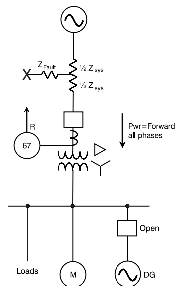
Fig. 8. System One-Line
