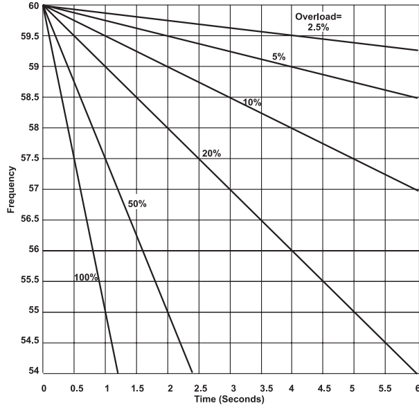
Figure 3a: Simple Analysis Frequency Decay, H=6 , Various P_a
