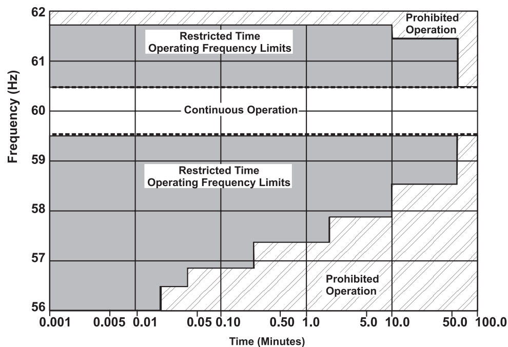
Figure 9: IEEE C37-106 Worst Case Frequency Withstand
