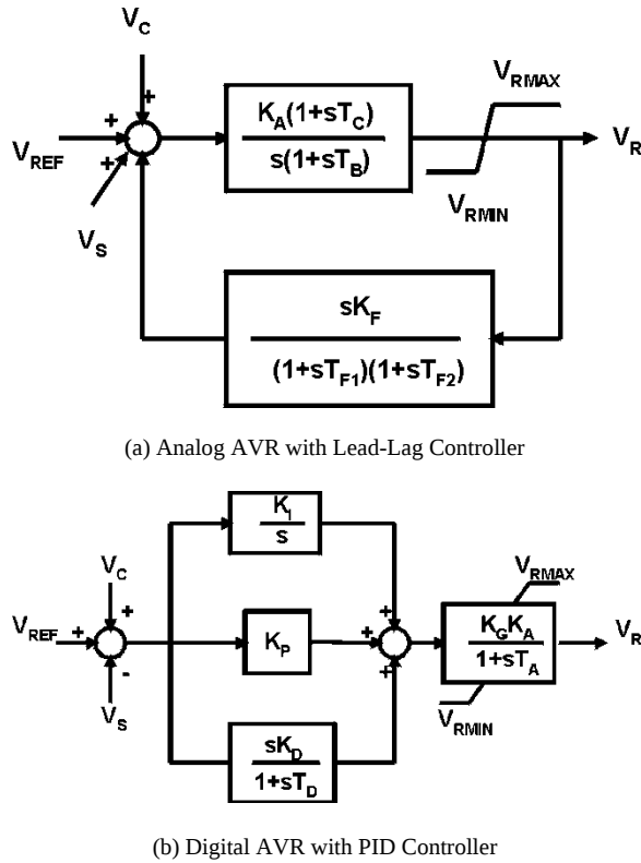
Fig. 3. Simplified Block Diagrams of Automatic Voltage Regulators
