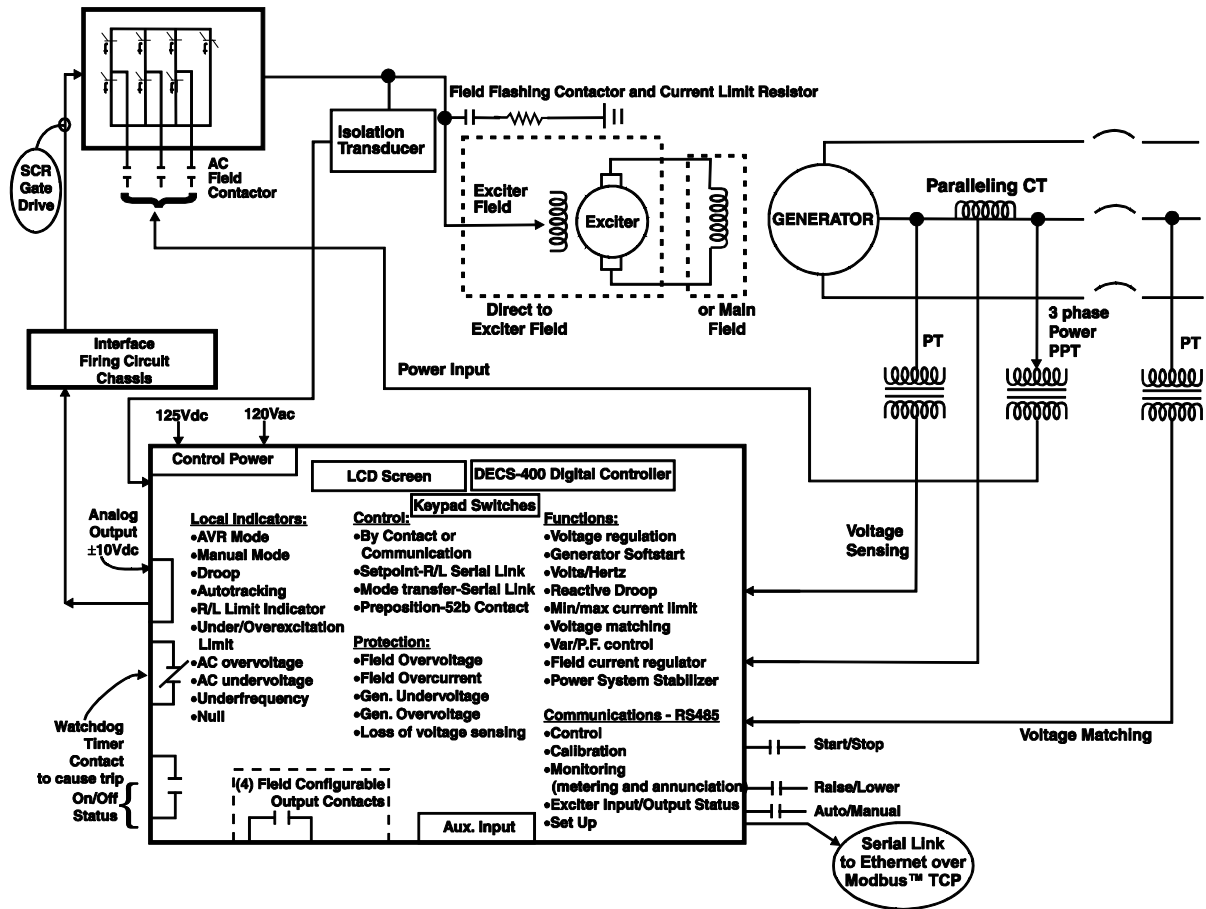
Fig. 2. A Typical Digital Excitation Control System
