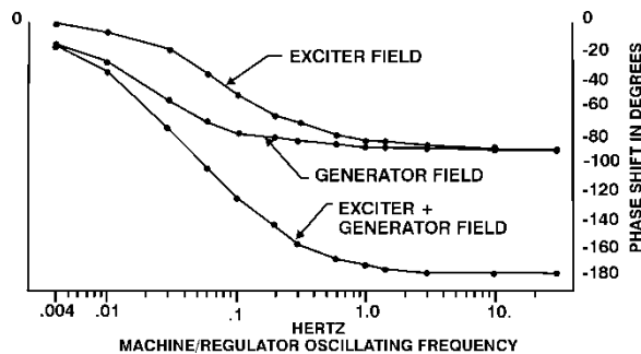
Fig. 11. Phase Shift of the Exciter Field, the Generator Field, and the Sum of the Two
