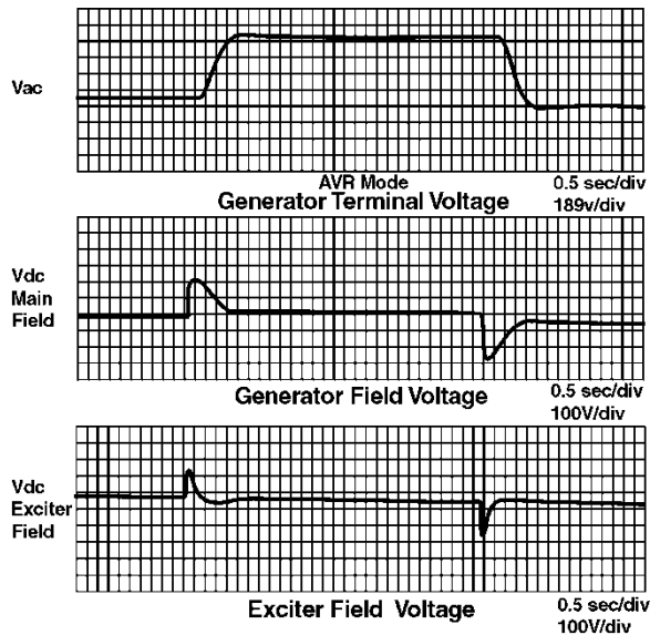
Fig. 10. Further Improvements With Gain Settings Increasing Derivative (KD)
