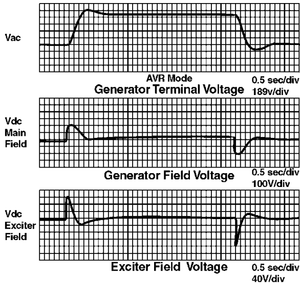
Fig. 8. Increased PID Gains
