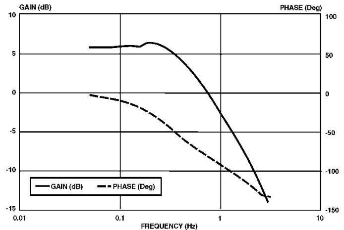
Fig. 13. Bode Plot of Off-Line Frequency Response with Digital Voltage Regulator
