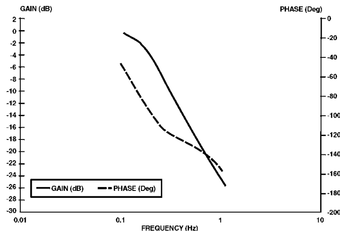
Fig. 12. Bode Plot of Off-Line Frequency Response with Analog Voltage Regulator
