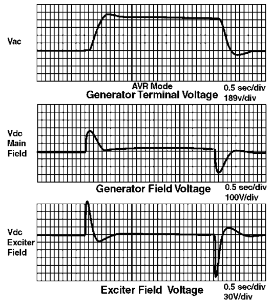
Fig. 9. Performance Variation with Modified P+D Settings
