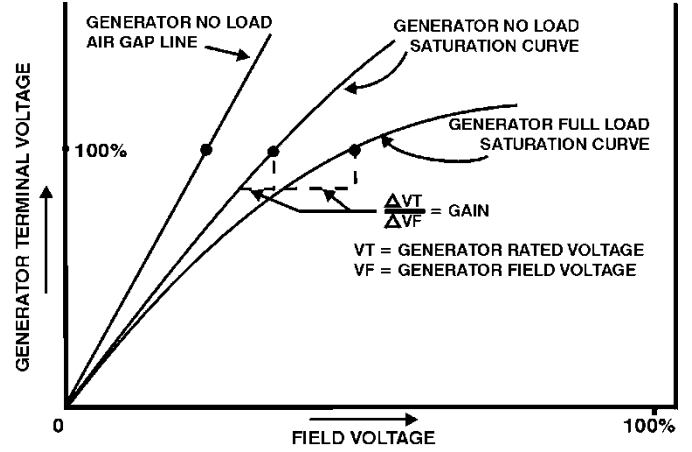
Fig. 4. Generator Saturation Curve Illustrating Generator Gain
