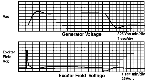
Fig. 5. Voltage Step Responses Performed on a Hydro Turbine Generator with Analog Voltage Regulation
