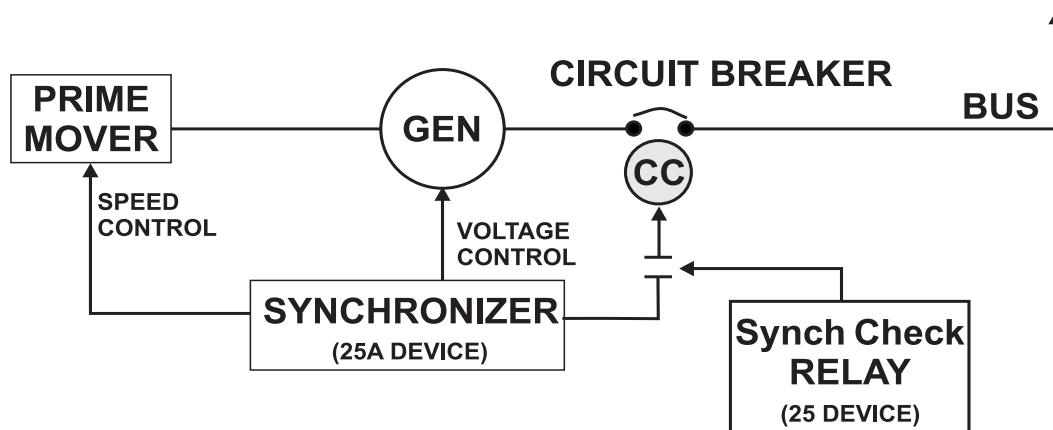
Figure 8: Automatic Synchronizing
